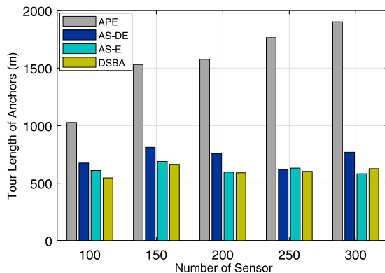
Fig. 8. Comparison of tour length of anchors.
